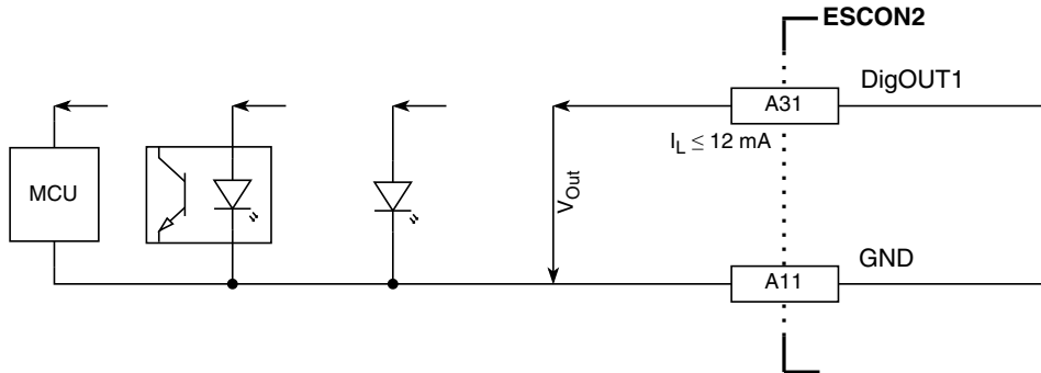
Figure 3-20 Wiring examples for "sourcing" on DigOUT1 (analogously valid for DigOUT2)
