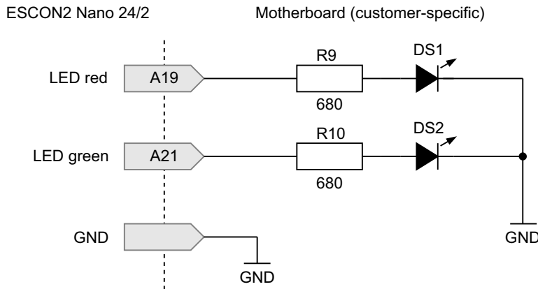
Figure 4-36 Wiring of LEDs for device status indication
