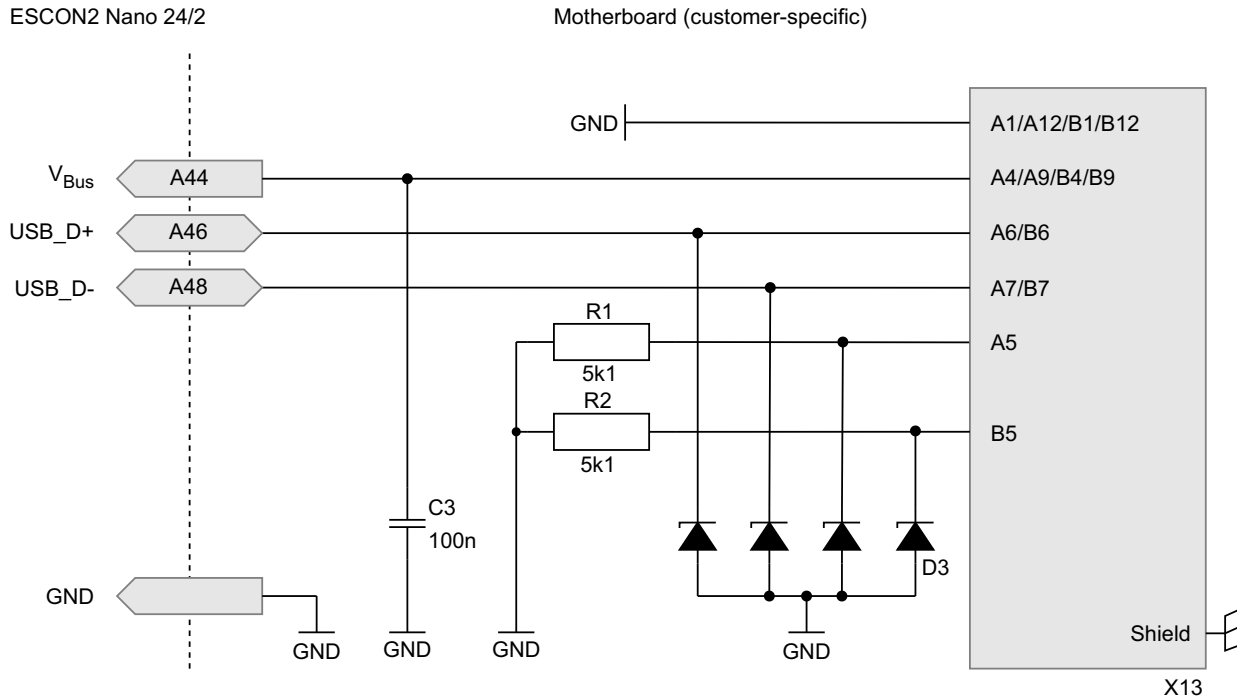
Figure 4-29 Wiring of USB-C connector
