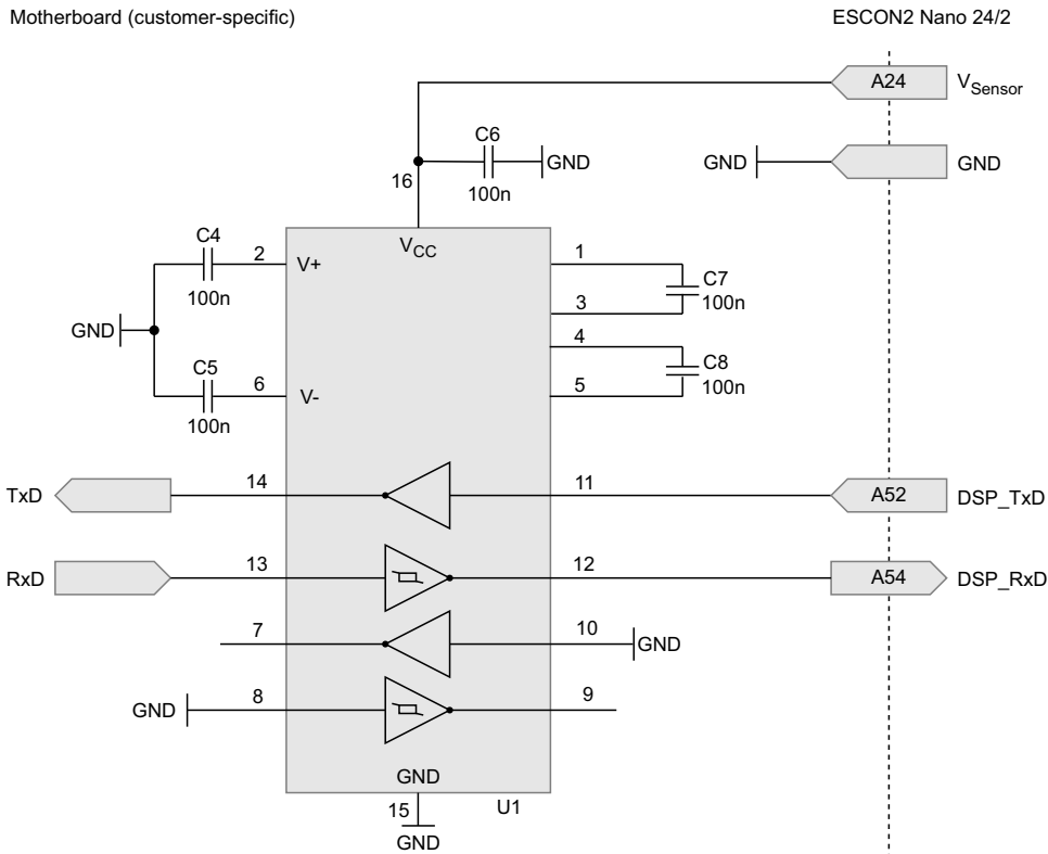
Figure 4-32 Wiring of RS232 interface
