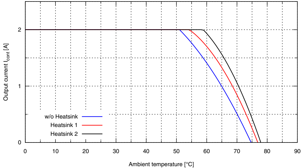
Figure 2-3 Extended operation @ V_{CC} 24 VDC with additional heatsink
