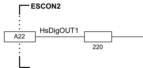
Figure 3-14 HsDigOUT1 circuit
