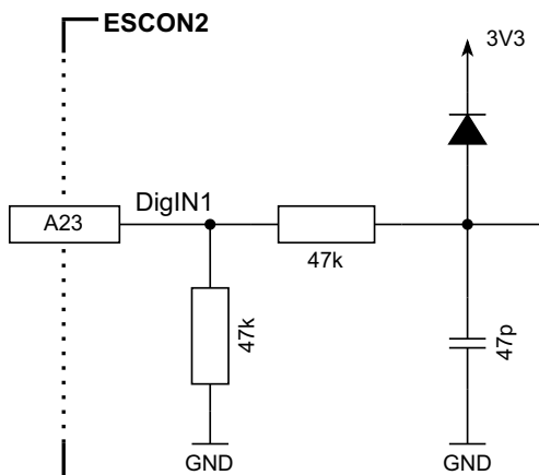
Figure 3-16 DigIN1 circuit (analogously valid for DigIN2)
