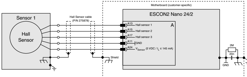
Figure 5-43 Sensor 1 Hall sensor
