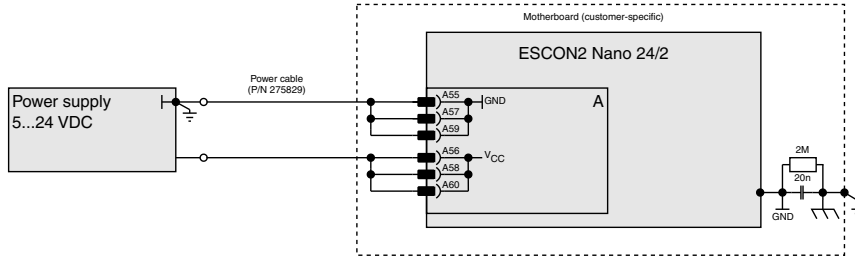
Figure 5-40 Power supply
