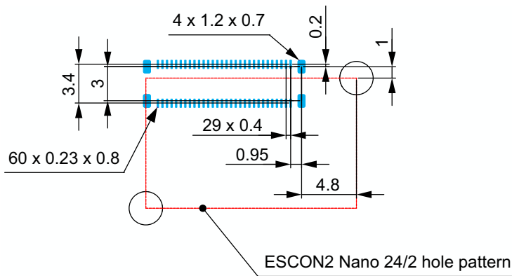
Figure 4-37 SMT footprint [mm] – Top view
