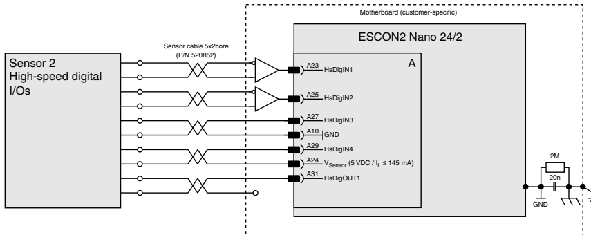
Figure 5-46 High-speed digital I/Os
