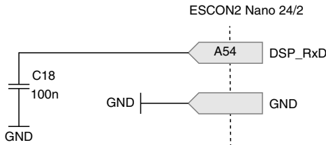
Figure 4-31 Wiring of Serial Communication Interface (SCI) not used
