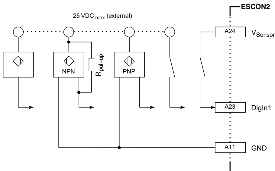
Figure 3-18 Wiring examples for proximity sensors and switches on DigIN1 (analogously valid for DigIN2..4)
