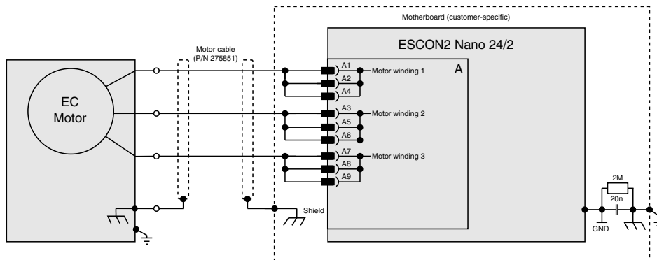
Figure 5-42 EC (BLDC) motor
