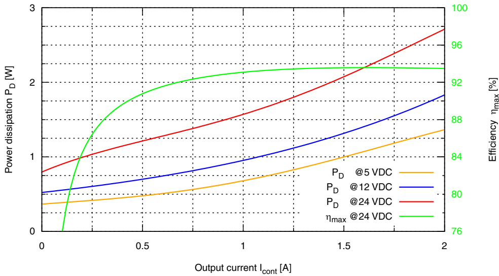
Figure 2-5 Power dissipation and efficiency
