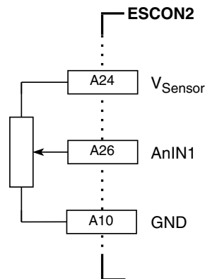
Figure 3-22 Wiring examples for a potentiometer on AnIN1 (analogously valid for AnIN2)
