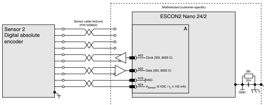
Figure 5-45 SSI / BiSS C unidirectional absolute encoder
