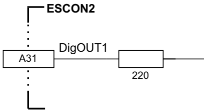
Figure 3-19 DigOUT1 circuit (analogously valid for DigOUT2)
