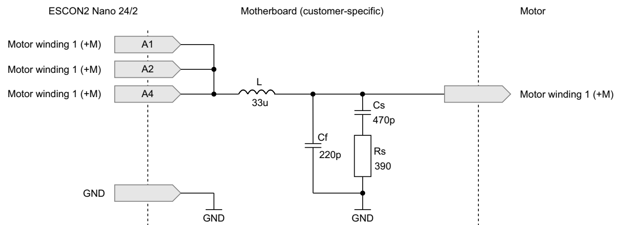
Figure 4-28 Wiring of motor winding 1 (analogously valid for motor winding 2 & 3)
