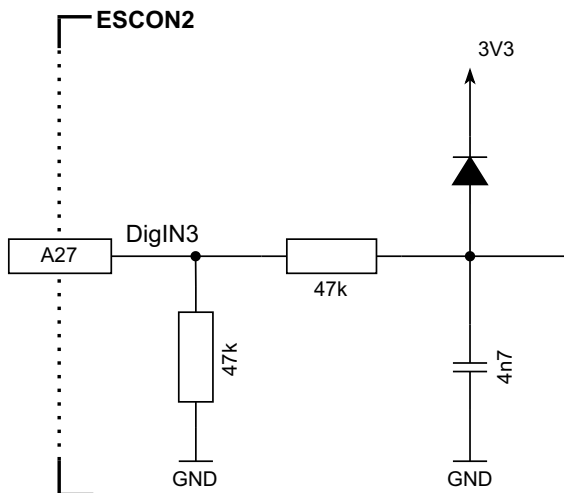
Figure 3-17 DigIN3 circuit (analogously valid for DigIN4)
