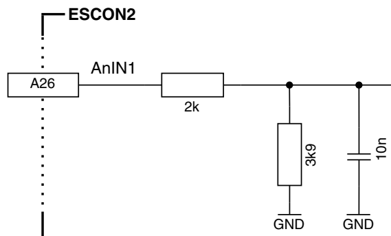
Figure 3-21 AnIN1 circuit (analogously valid for AnIN2)
