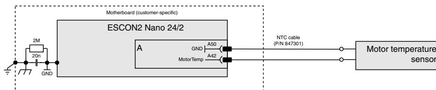
Figure 5-53 Motor temperature sensor
