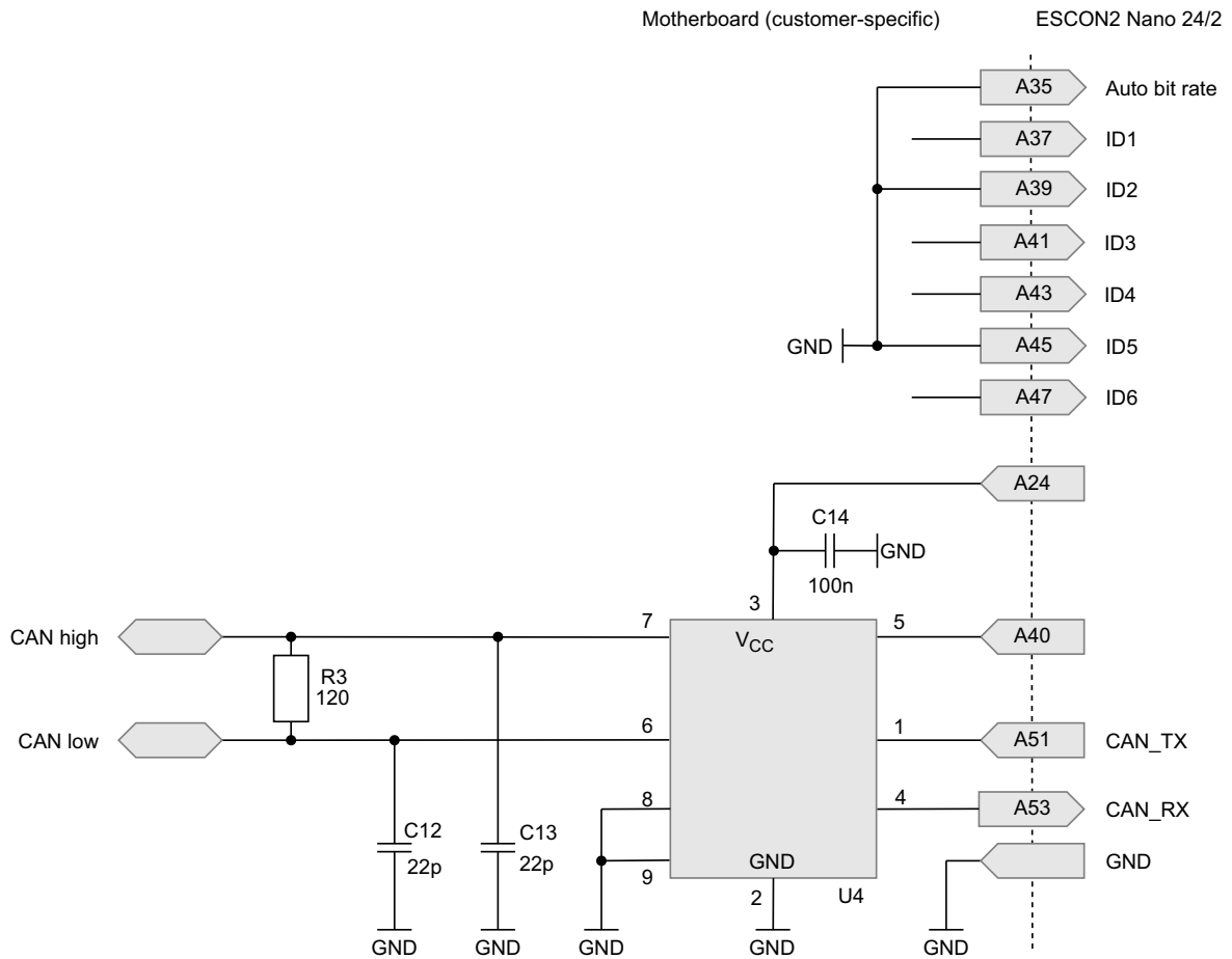
Figure 4-30 Wiring of CAN interface
