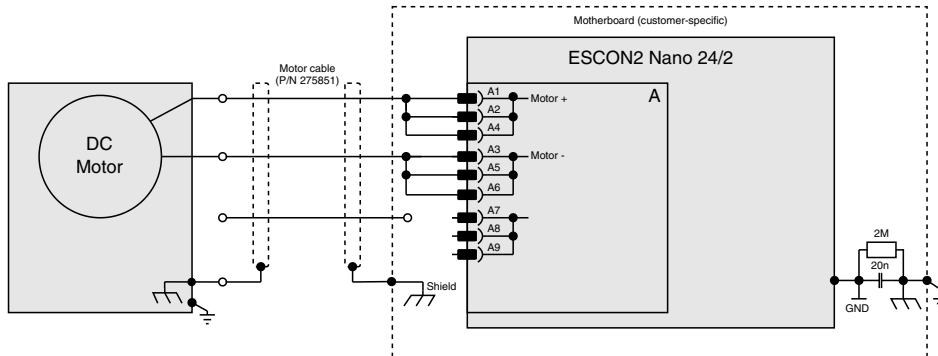
Figure 5-41 DC motor
