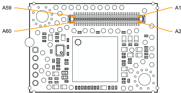
Figure 5-38 Interfaces – Designations and location
