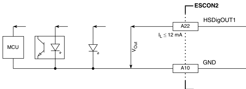
Figure 3-15 Wiring examples for "sourcing" on HsDigOUT1
