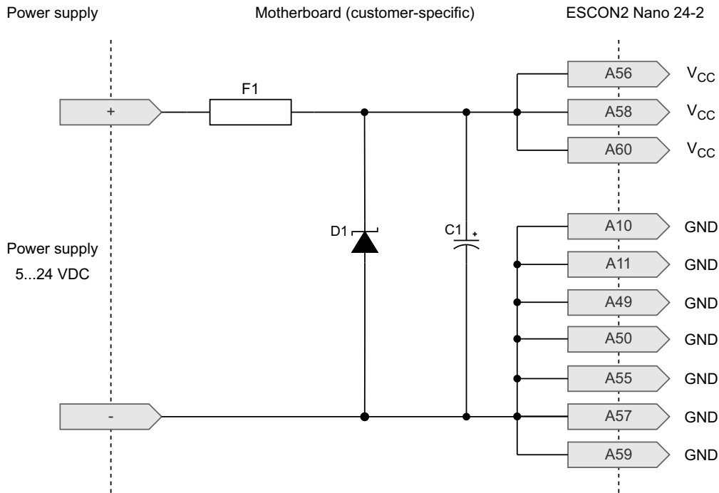
Figure 4-27 Wiring of power supply
