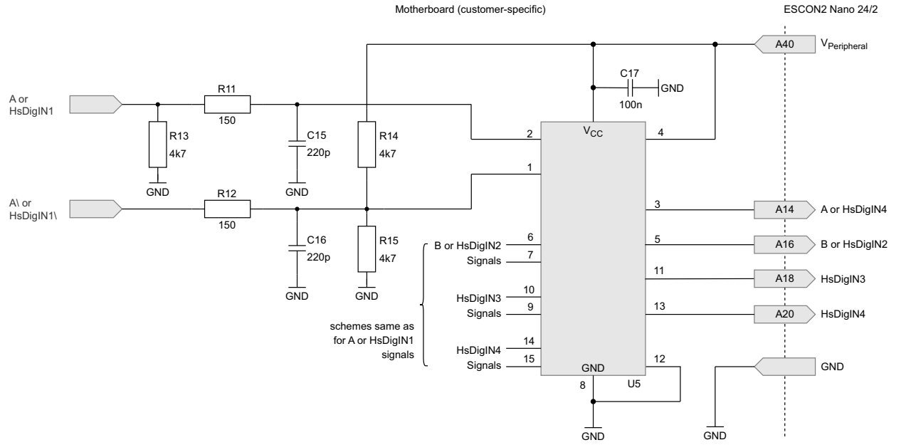
Figure 4-33 Wiring of RS422 line receiver for incremental encoder or high-speed I/O signals
