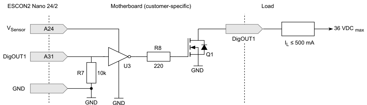
Figure 4-35 Wiring of digital output 1 load switch (analogously valid for digital output 2)
