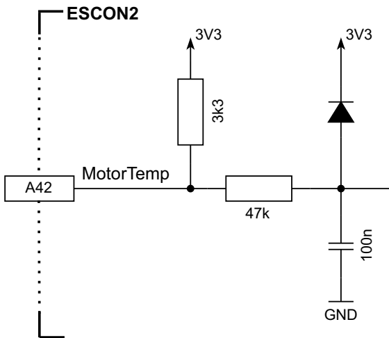
Figure 3-25 Motor temperature circuit
