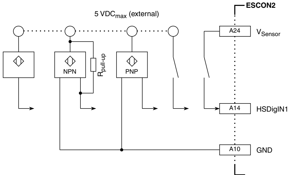
Figure 3-13 Wiring examples for proximity sensors and switches on HsDigIN1 (analogously valid for HsDigIN2..4)
