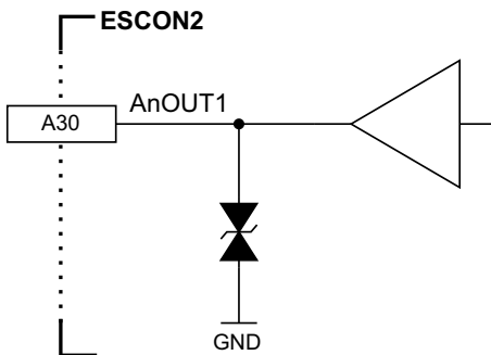
Figure 3-23 AnOUT1 circuit (analogously valid for AnOUT2)
