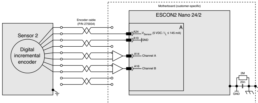
Figure 5-44 Digital incremental encoder
