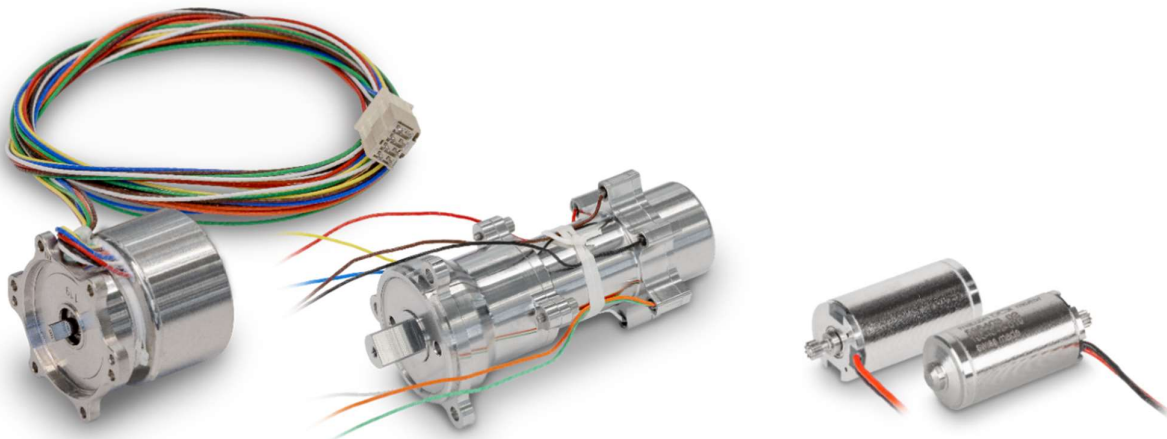
Left: The modified EC 32 flat drive, nine of these drives are used in the Perseverance rover.
