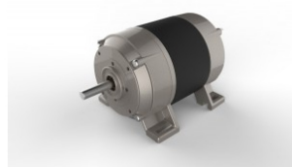
SD28 Family Torque 0.37 - 0.4 Nm Speed 1400 - 2800 RPM Power 55 - 120 Watts Voltage 24V - 440V
